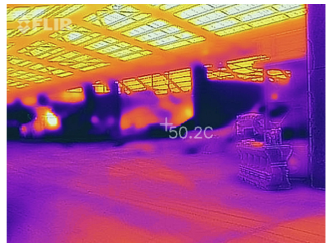
Fig. 8. Concentrate bagging shed. Significance of radiant heat from un-insulated corrugated iron roof visible in thermal gradient. The dark areas are walls retaining the concentrate (in granular form). 50.2 °C of the selected area is the surface temperature of the concentrate. The roof is hotter, as demonstrated in the next image.
